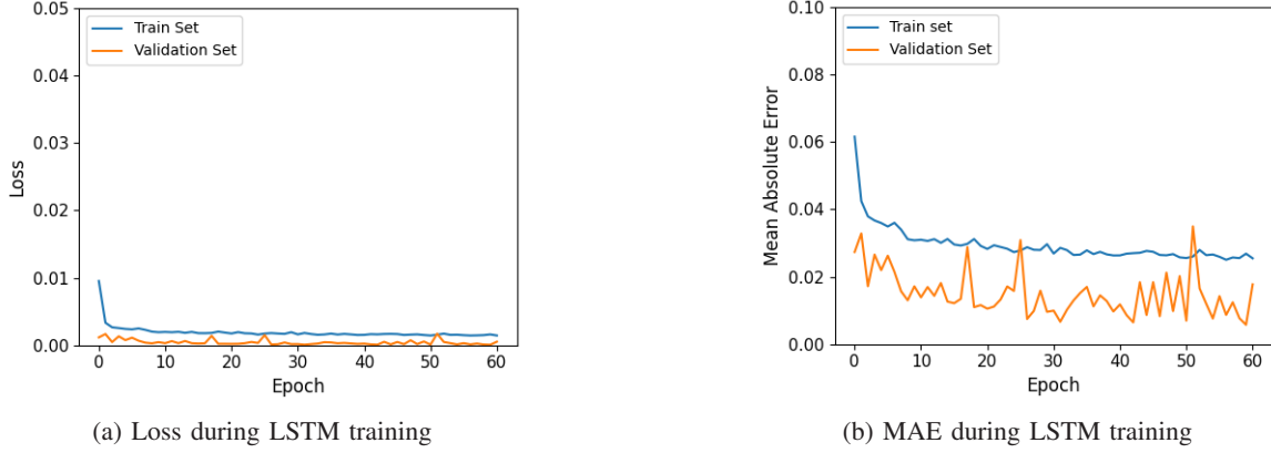
Fig. 7: Loss and MAE of the LSTM model during the training process
