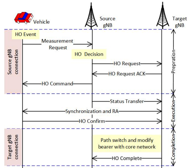
Fig. 1: Handover procedure
